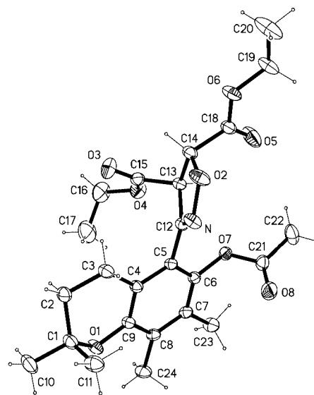
Figure 3. Thermal ellipsoid plot (25% ellipsoids) and crystallographic atom labeling of tocopherylisoxazoline 8
