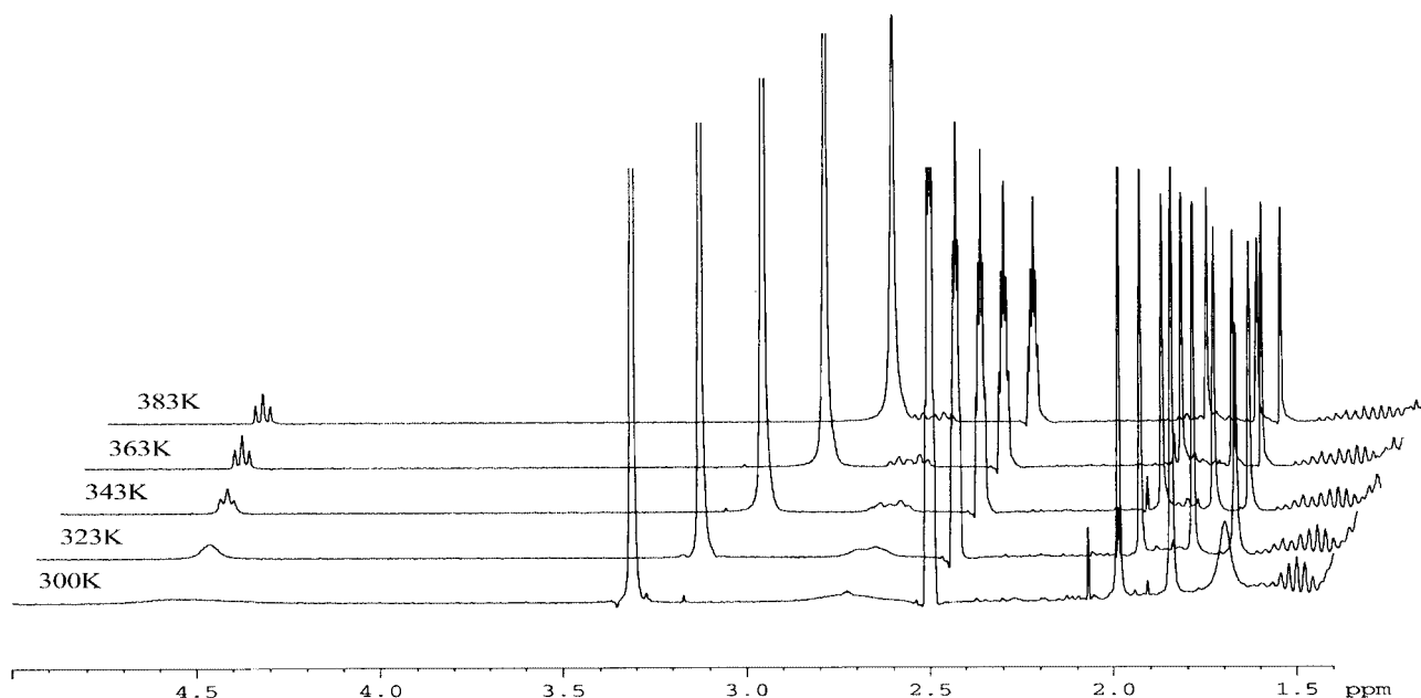
Figure 4. Stacked plots of ^1\text{H} NMR spectra (region between \delta = 1.5 and 5.0 ppm) of isoxazoline 6 , recorded at different temperatures in [\text{D}_6]\text{DMSO} ; note the temperature-dependent line shape and chemical-shift changes of the resonances of 4''\text{-CH} ( \delta \approx 4.5 ppm), 4\text{-CH}_2 ( \delta \approx 2.6\text{--}2.8 ppm) and the acetyl group ( \delta \approx 1.6\text{--}1.8 ppm)
