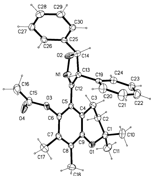
Figure 1. Thermal ellipsoid plot (20% ellipsoids) and crystallographic atom labeling of tocopherylisoxazoline 6 (4,5-diphenyl substituents in trans configuration)
