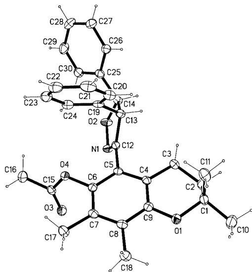
Figure 2. Thermal ellipsoid plot (40% ellipsoids) and crystallographic atom labeling of tocopherylisoxazoline 9 (4,5-diphenyl substituents in cis configuration) showing only one of the two conformationally different independent molecules
